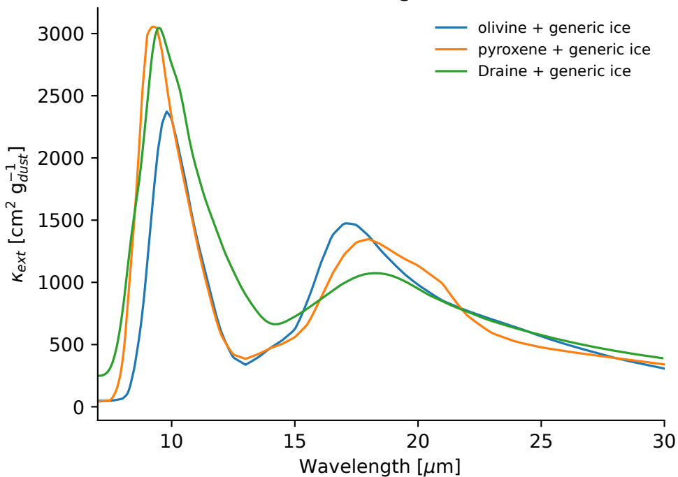
A. Isolated coated-grain extinction
