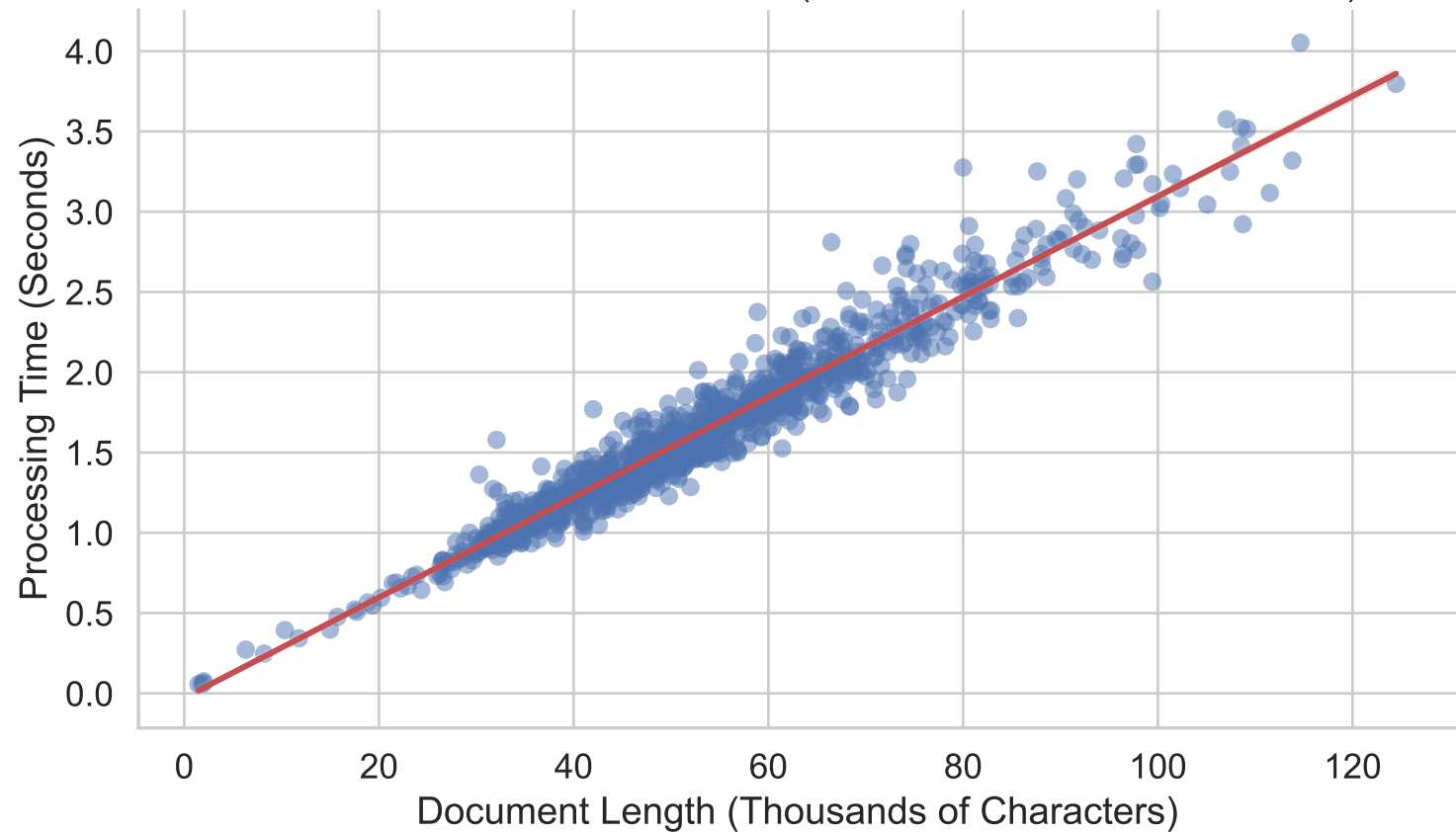
Tier D: Parser Scale Robustness (n=1000 PDFs, Pearson r = 0.97)
