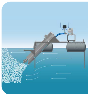
DualStar in Aeration Mode
