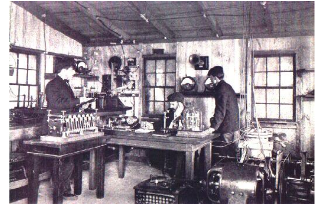
Labor von Fessenden in Brant Rock, Massachusetts, 1906
