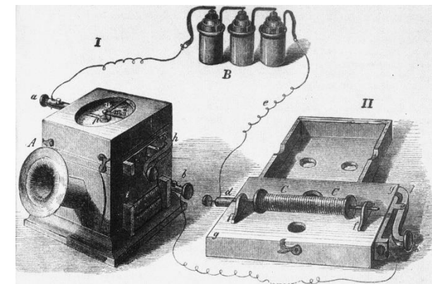
Reis'sches Telefon, 1863
