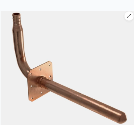
PX1290SO 1/2" X 8" Pex Stubout 90 W/ Bracket
