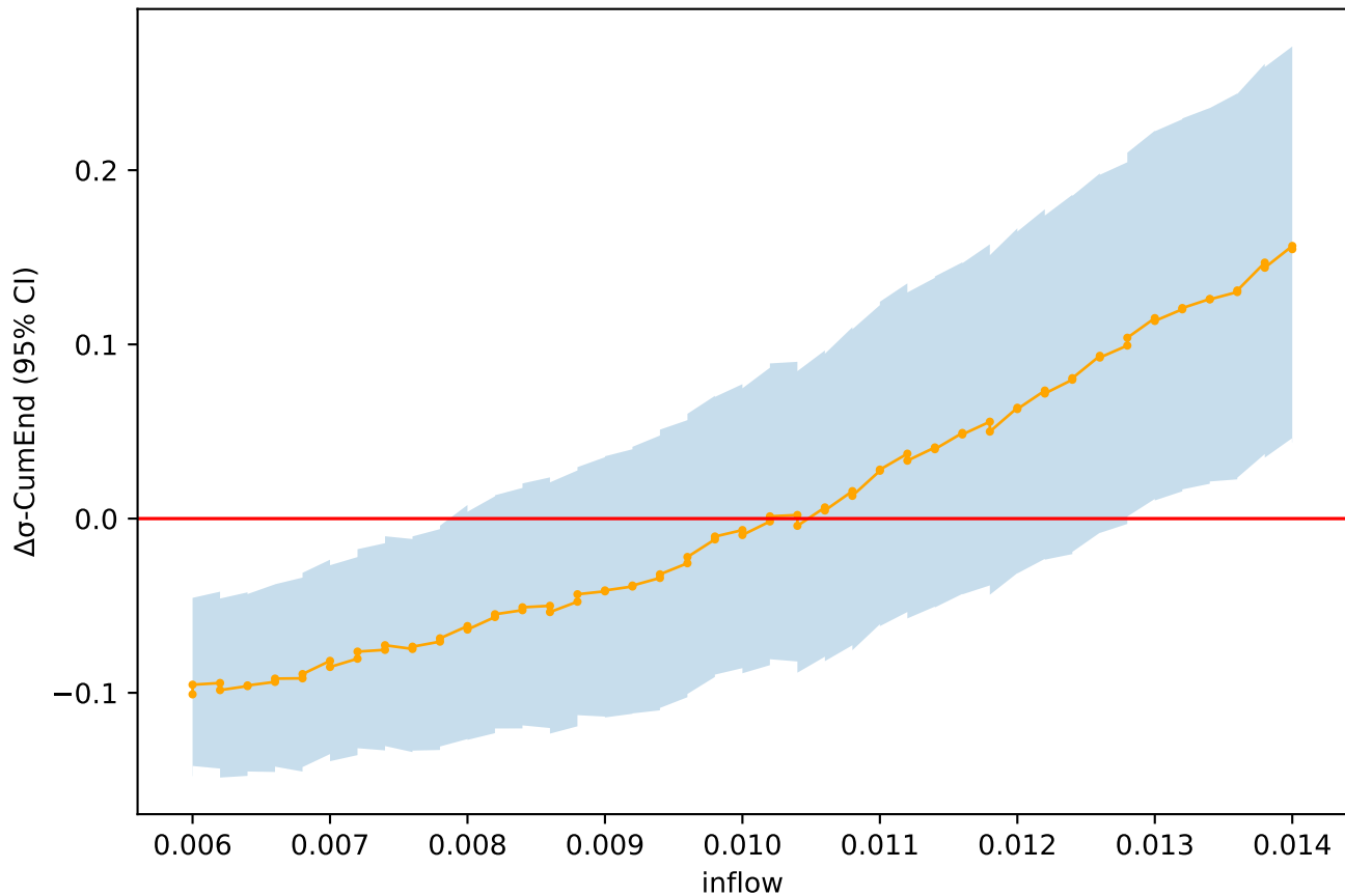
\Delta\sigma -CumEnd vs inflow (95% CI)
