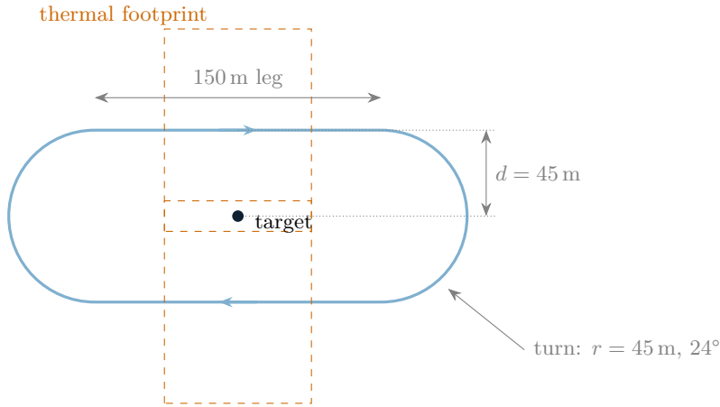
Figure 36: The closer look seen from above: a racetrack centred on the detection. The legs are flown wings level 45 m to either side, so the nadir thermal footprint (dashed) covers the target on every pass. The aircraft never flies over it, and the 24^\circ turns are made at the ends, away from the target.
