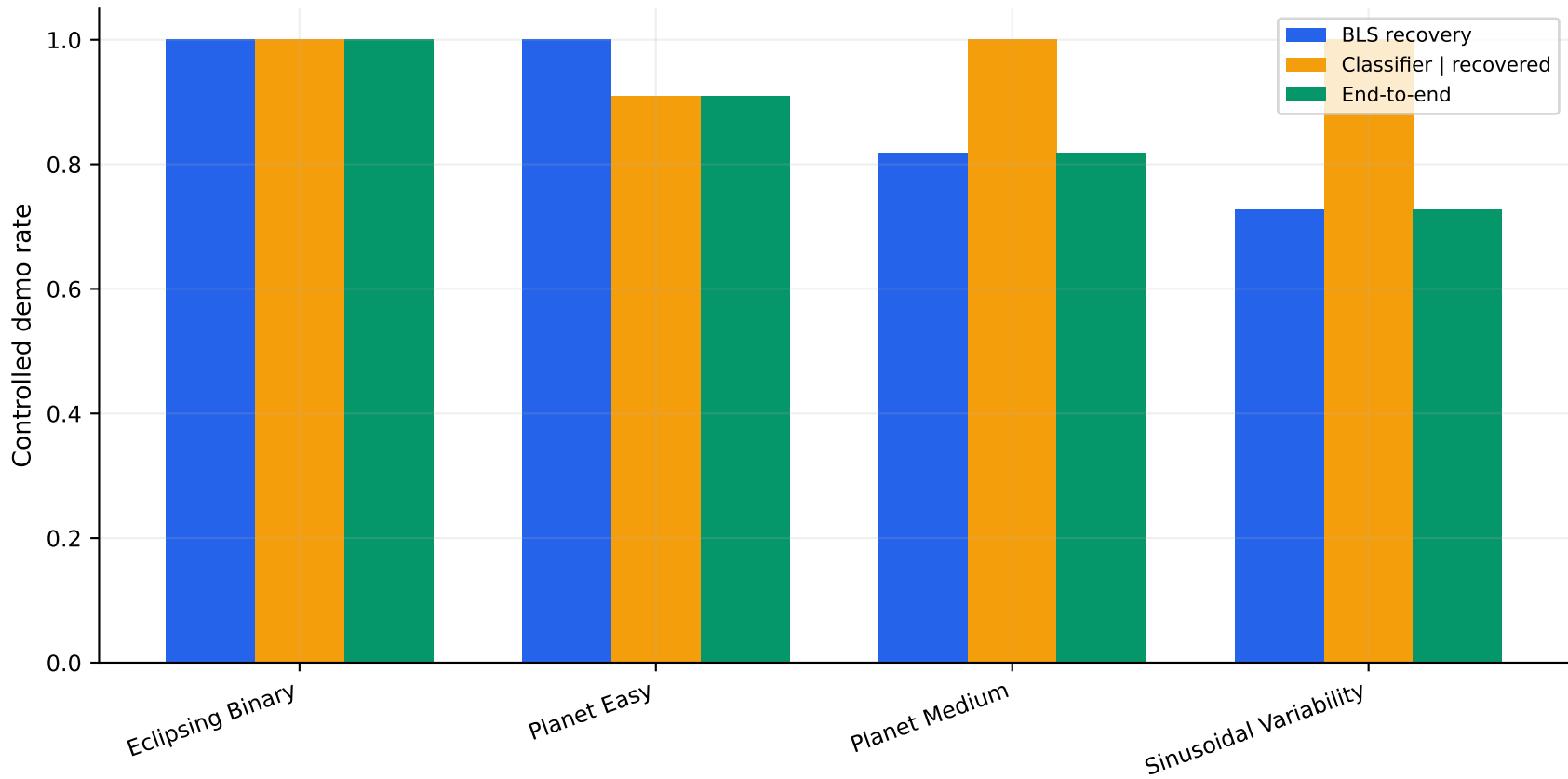
Synthetic-injection recovery stages
