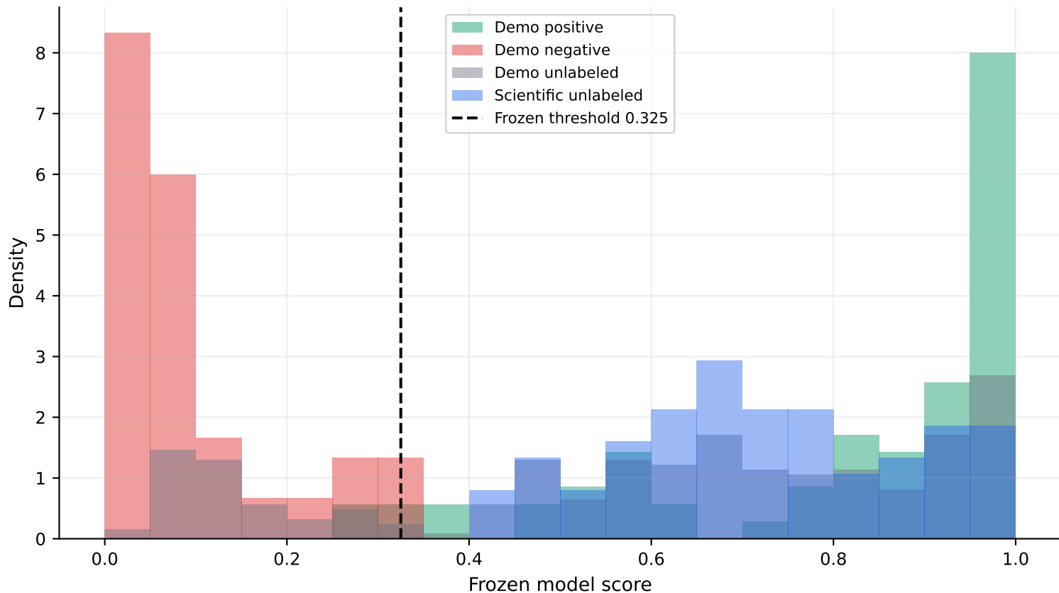
Demo and unlabeled scientific score distributions
