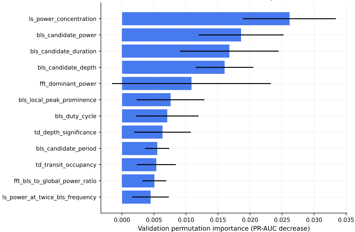
Frozen Random Forest feature importance
