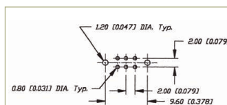
P.C. MOUNTING
