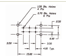
P.C. MOUNTING
