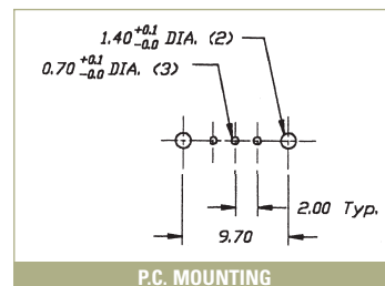
P.C. MOUNTING
