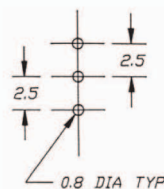
P.C. MOUNTING
