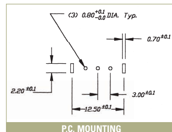
P.C. MOUNTING
