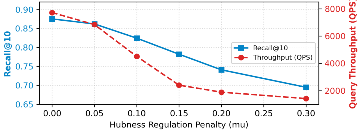
Hubness Regulation Sensitivity Sweep on Synthetic-Multi-Cluster (N=50K, D=64)
