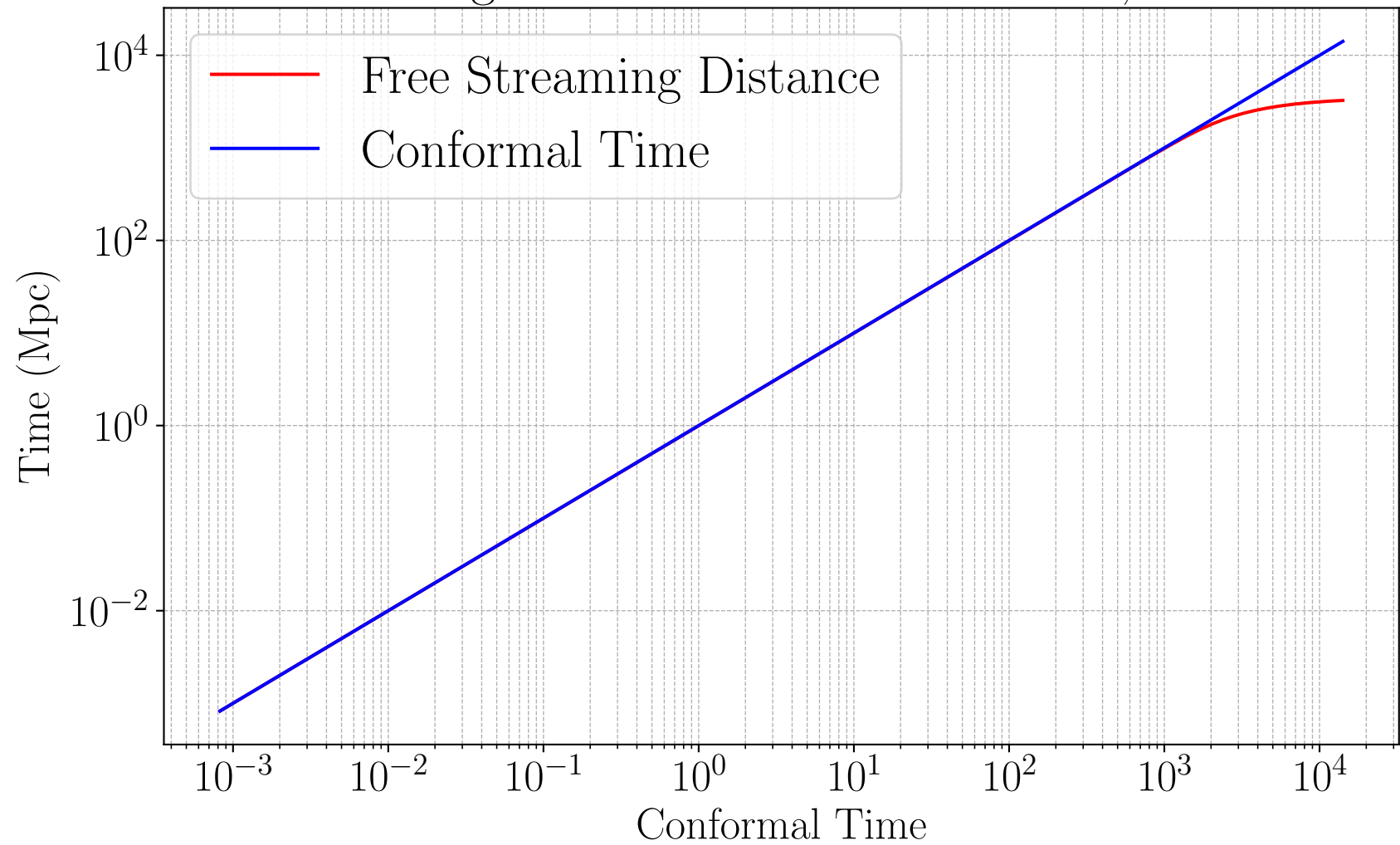
Free Streaming Distance vs Conformal Time, m = 0.06\text{eV}
