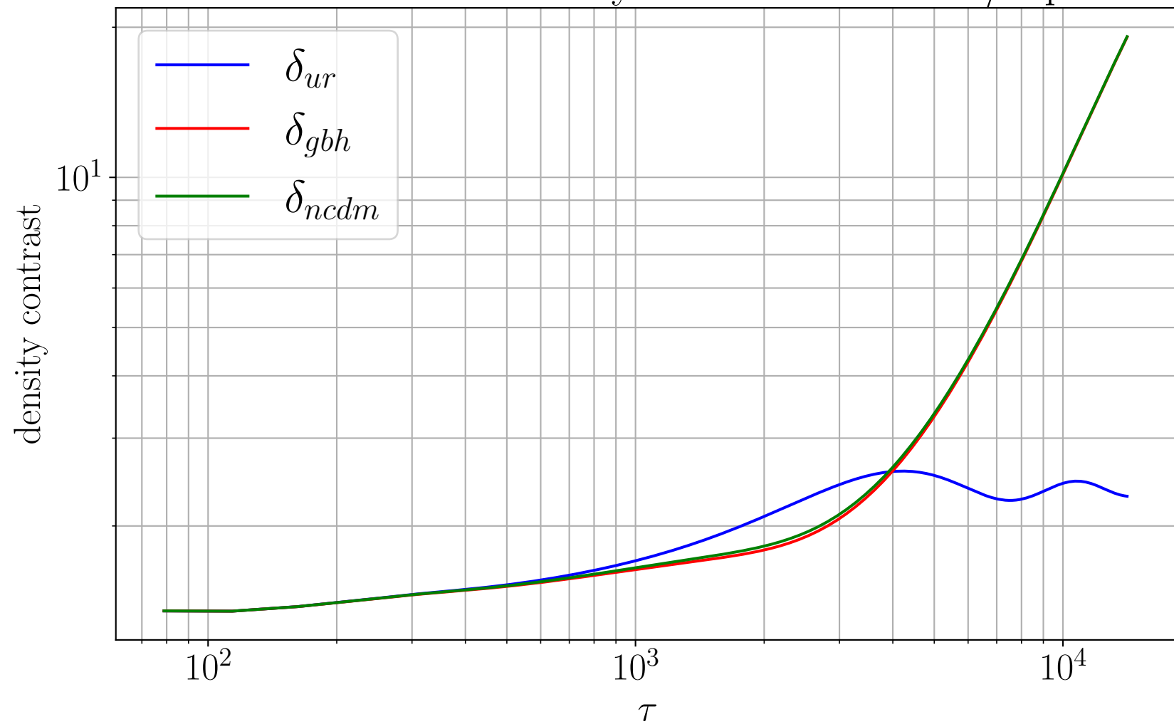
evolution of overdensity vs tau for k=0.001/\text{Mpc}
