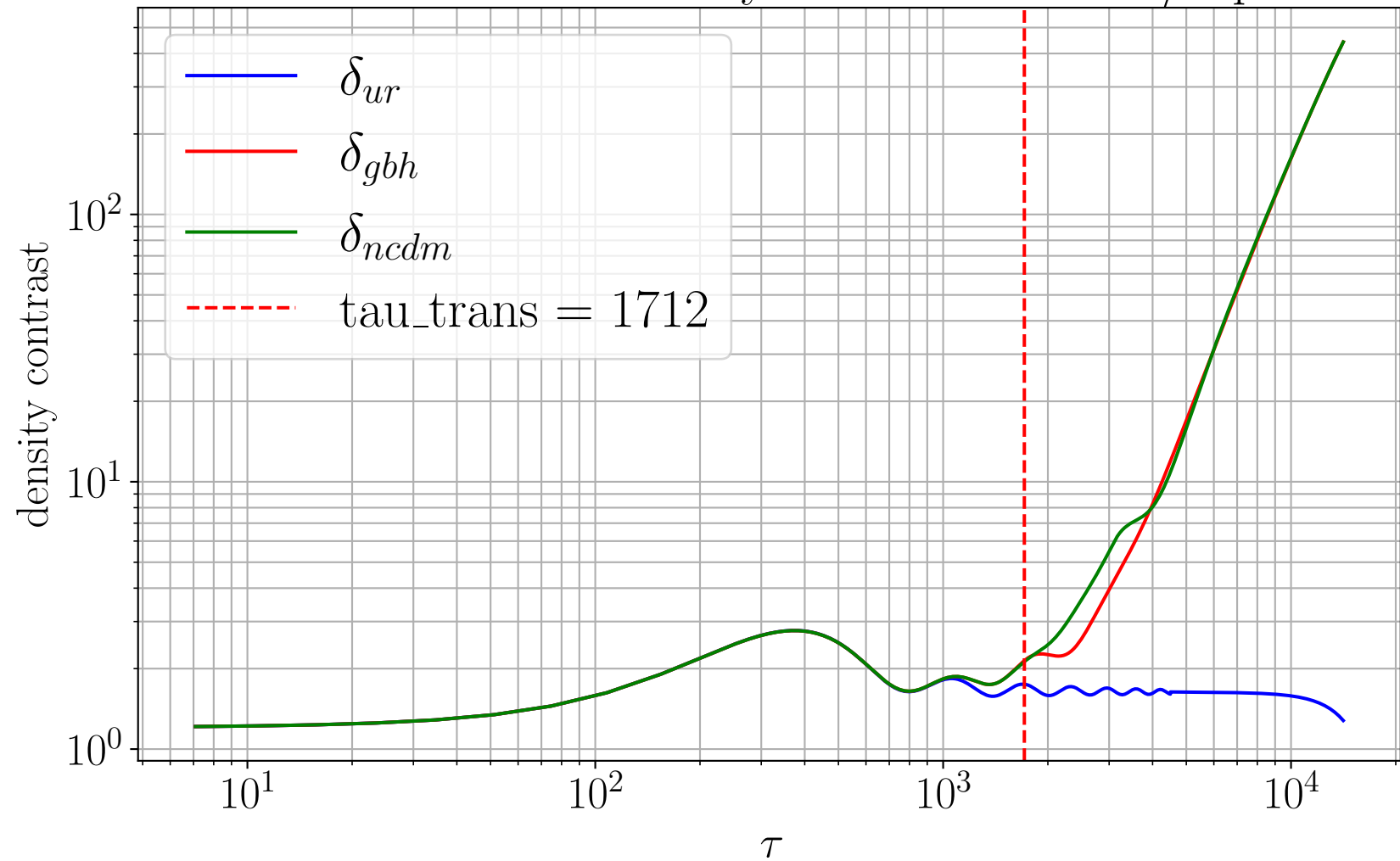
evolution of overdensity vs tau for k=0.01/\text{Mpc}
