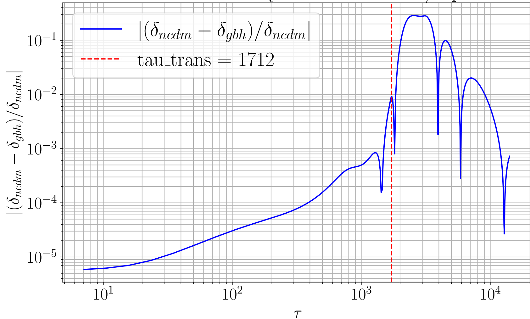
error in overdensity vs tau for k=0.01/\text{Mpc}
