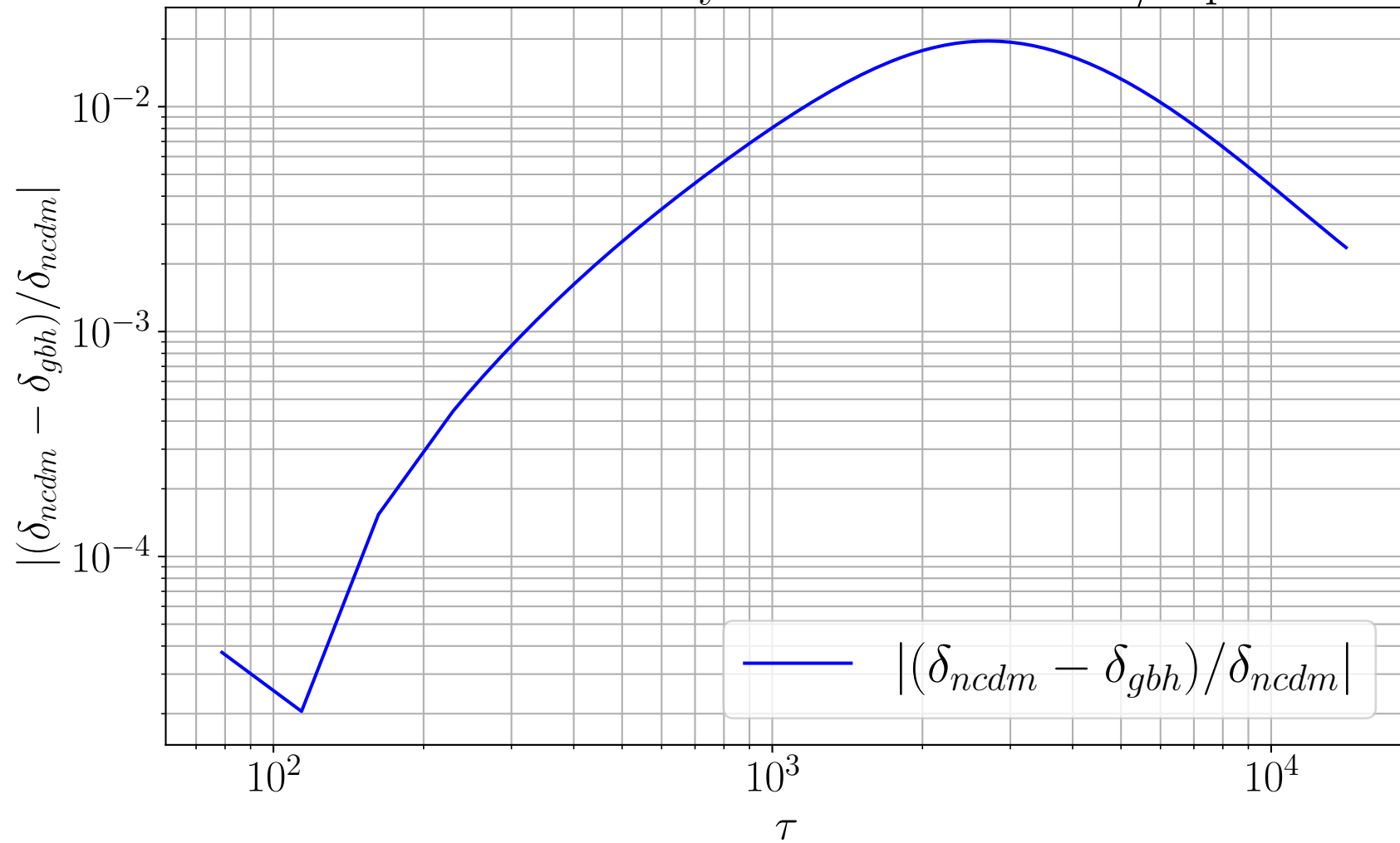
error in overdensity vs tau for k=0.001/\text{Mpc}
