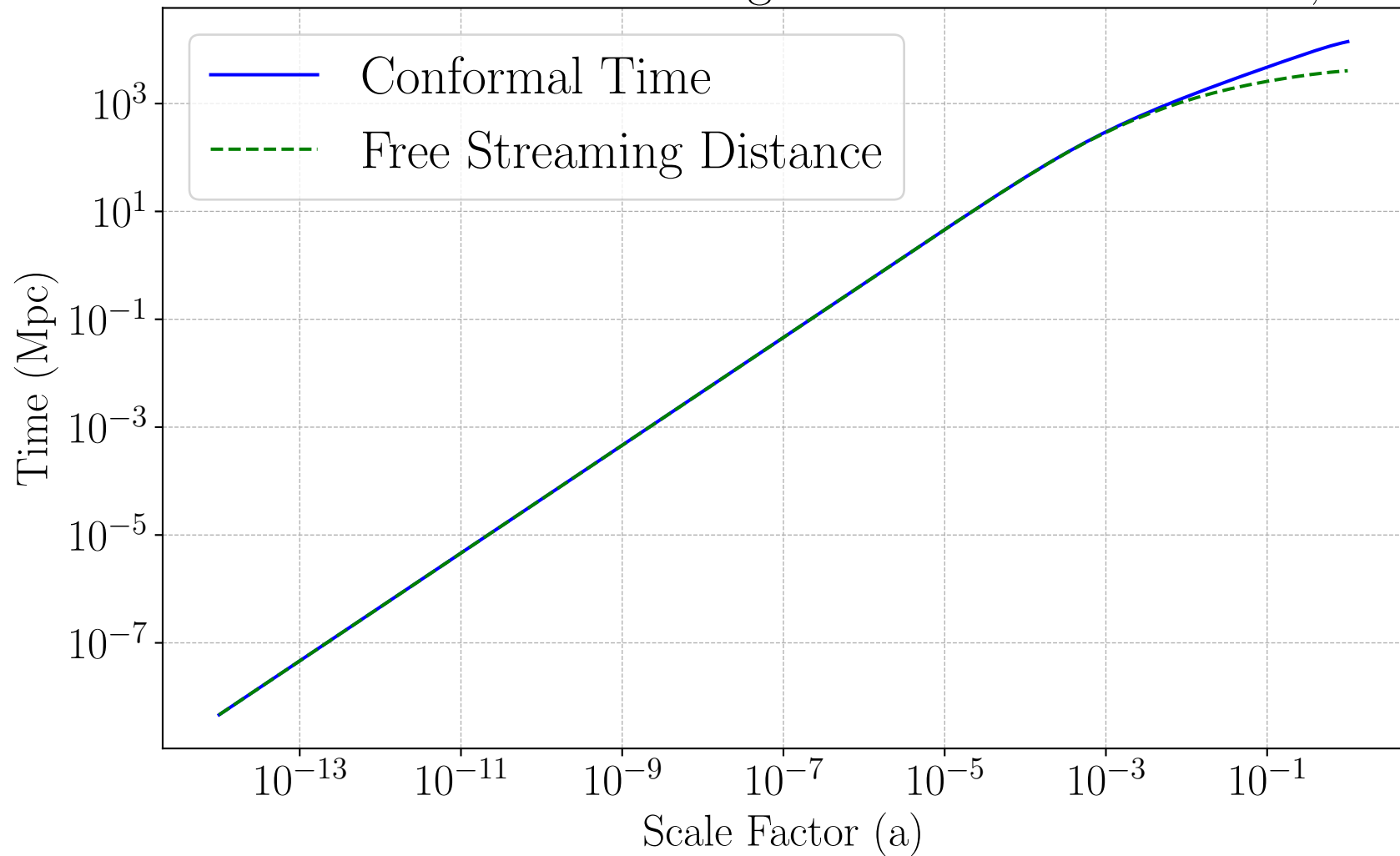
Conformal Time and Free Streaming Distance vs Scale Factor, m = 0.06\text{eV}
