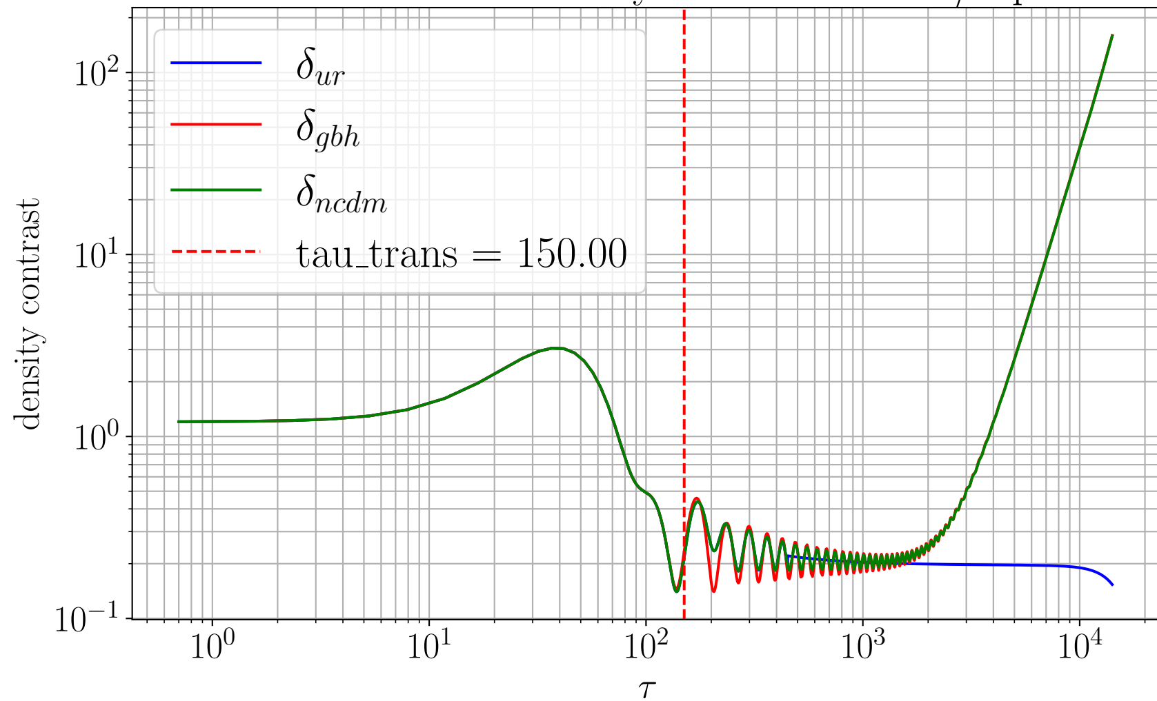
evolution of overdensity vs tau for k=0.1/\text{Mpc}
