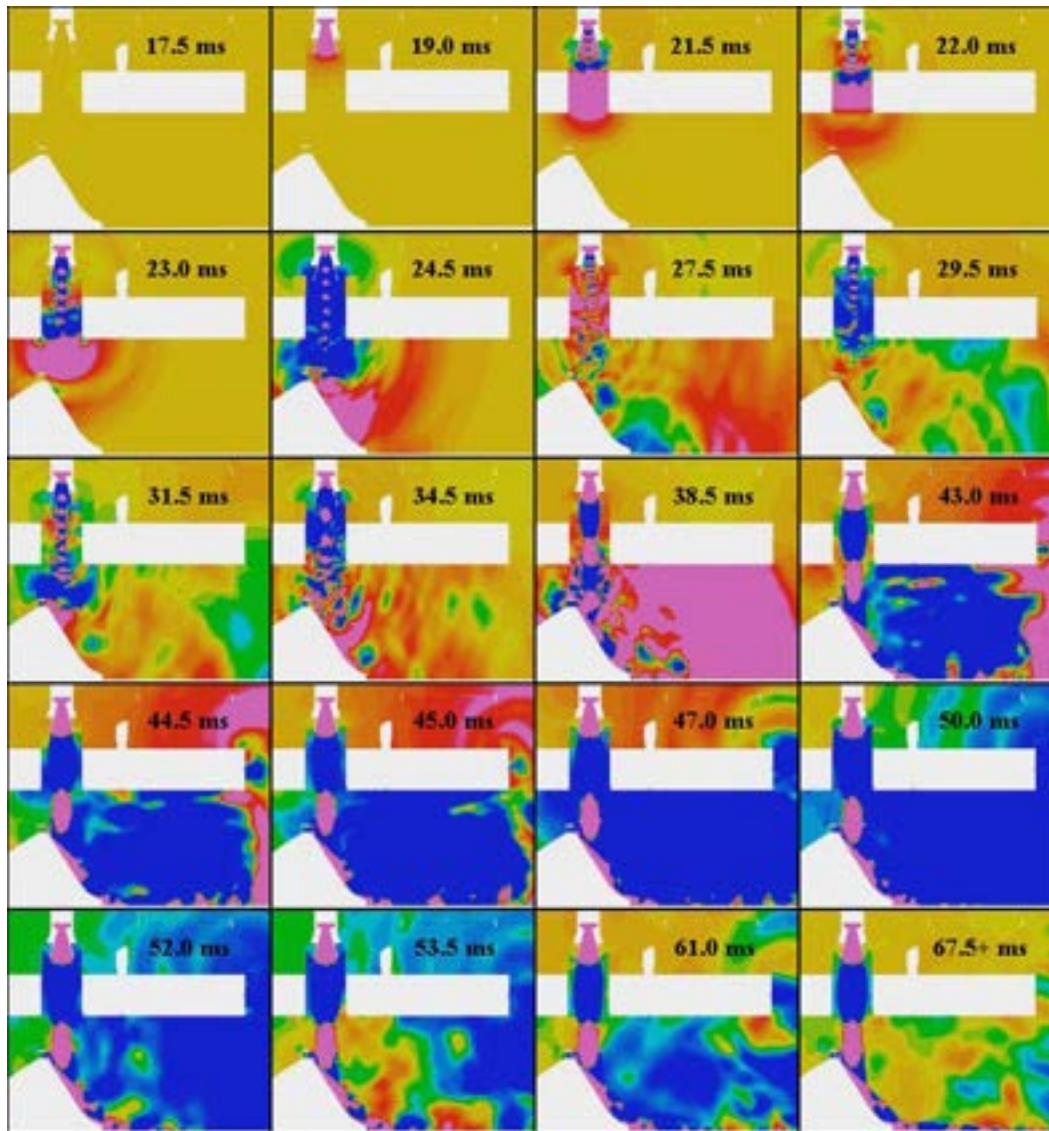
Figure 12 - Time Progression of Pressure Waves in Refined Pathfinder Simulation
