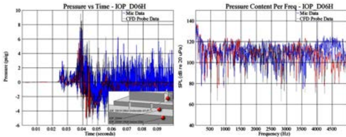
Figure 26 - Time and Frequency Comparison for Sensor IOP D06H (Refined Sim)
