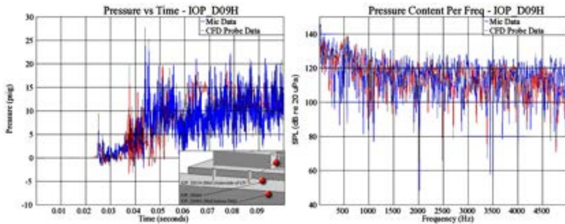
Figure 27 - Time and Frequency Comparison for Sensor IOP D09H (Refined Sim)
