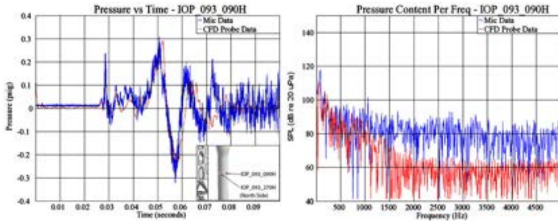
Figure 25 - Time and Frequency Comparison for Sensor IOP 093 090H (Refined Sim)
