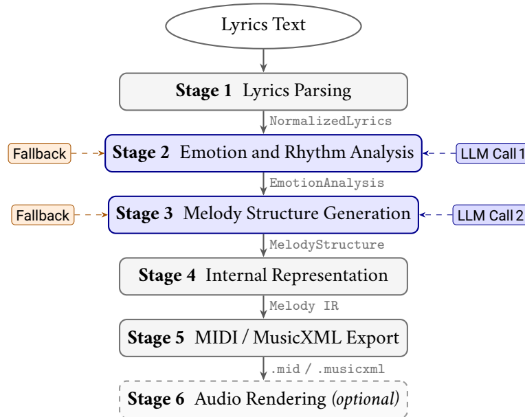
FIGURE 4.1. L2M six-stage sequential pipeline. Blue stages invoke LLM API calls; each has a deterministic fallback (orange). Stage 6 (dashed) is optional and requires FluidSynth.
