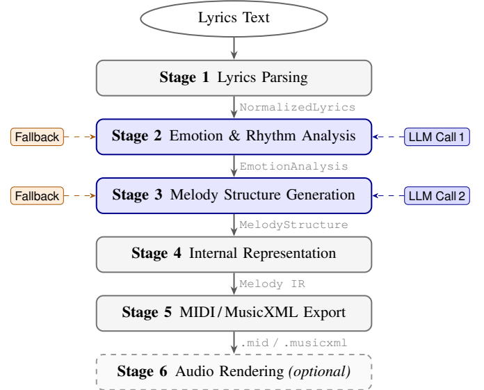
Fig. 1. L2M six-stage sequential pipeline. Blue stages invoke LLM API calls; each has a deterministic fallback (orange). Stage 6 (dashed) is optional and requires FluidSynth.
