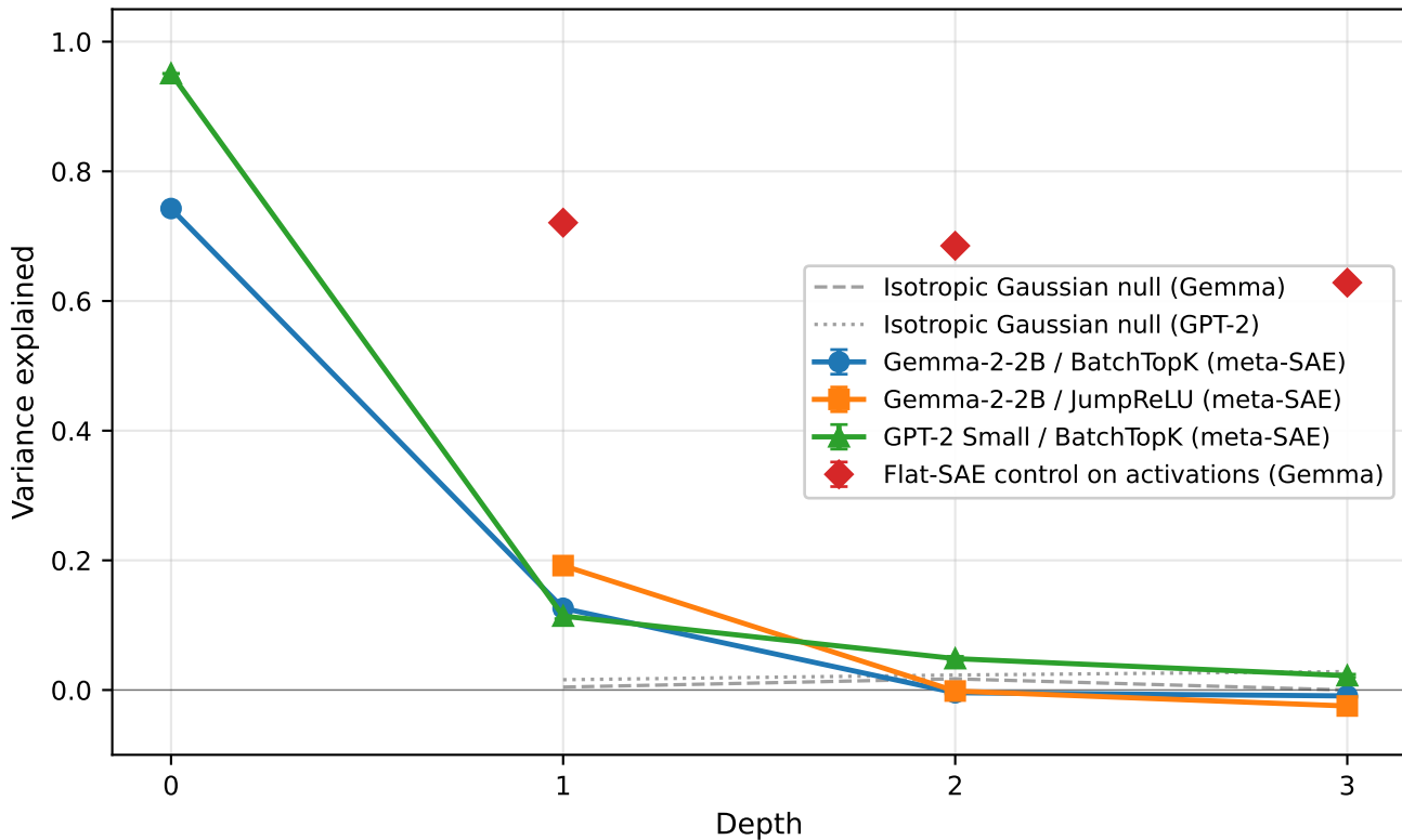
Variance explained by depth, audit-corrected (mean \pm std across seeds)
