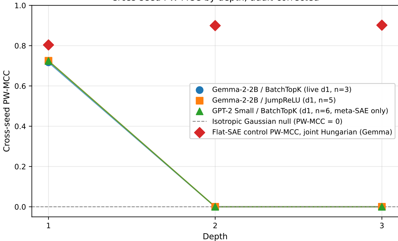
Cross-seed PW-MCC by depth, audit-corrected
