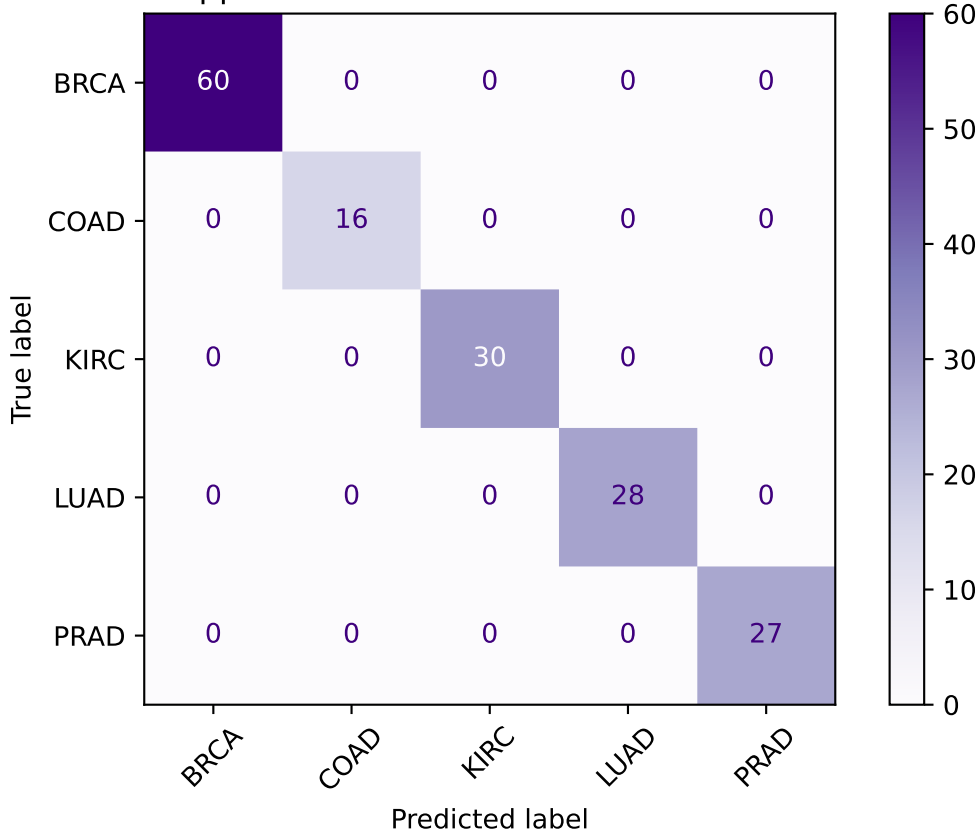
Support Vector Machine Confusion Matrix
