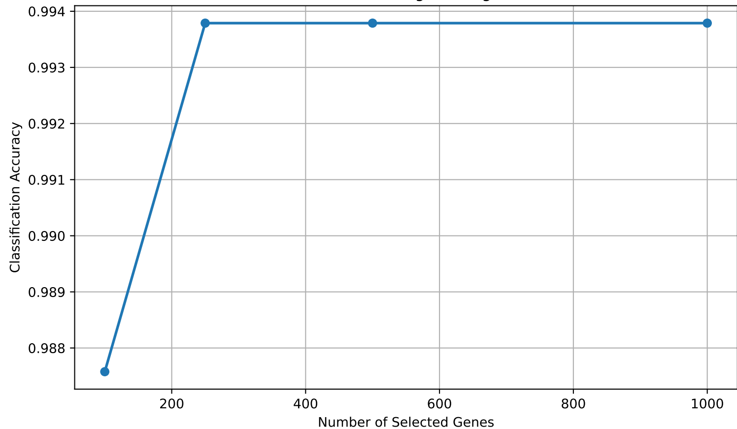
Effect of Feature Selection on Logistic Regression Performance
