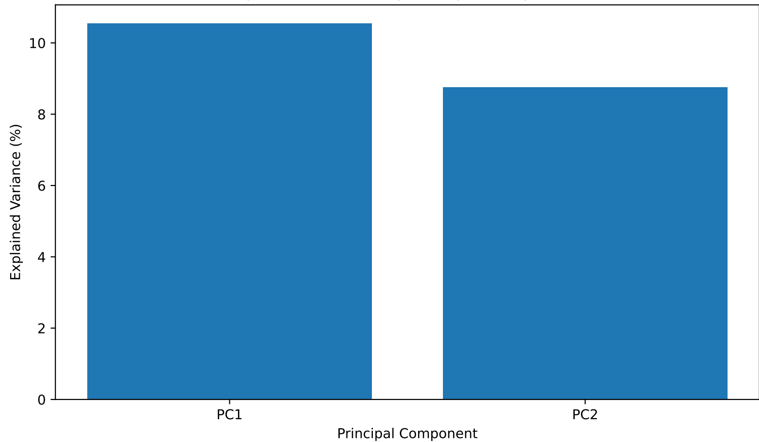
Explained Variance by Principal Components
