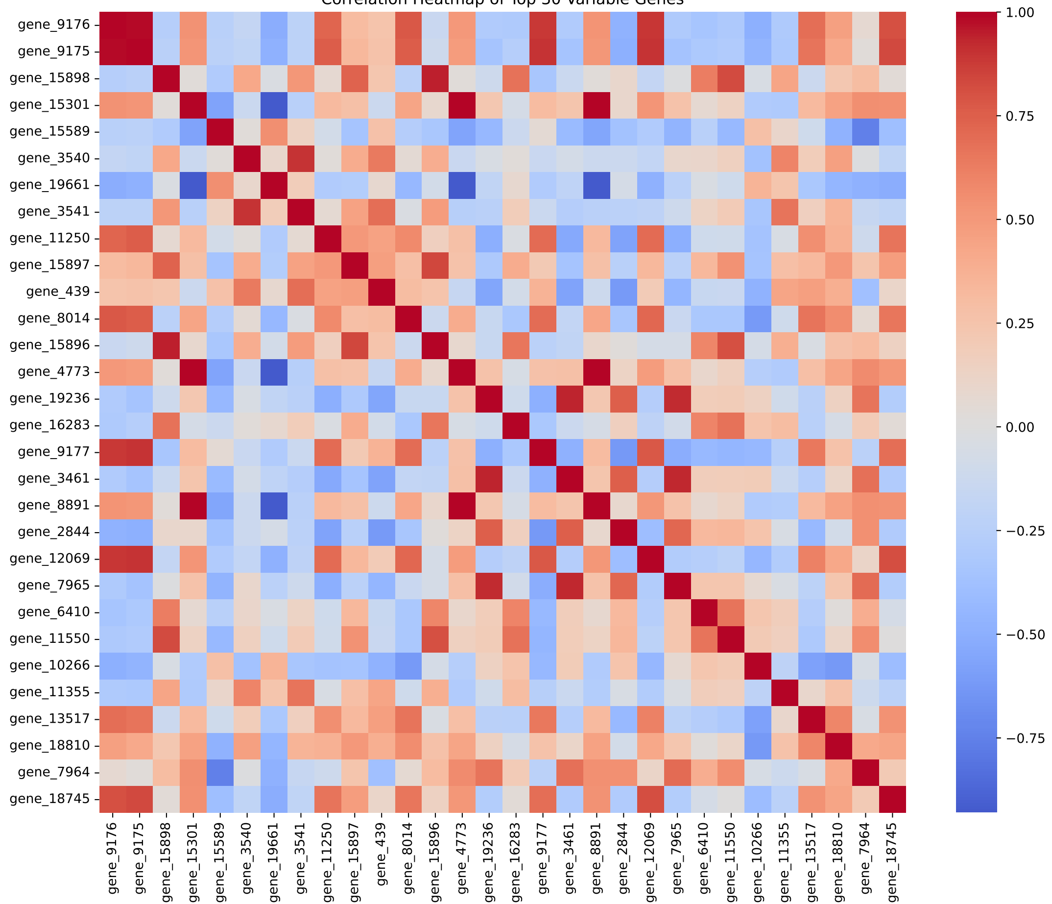
Correlation Heatmap of Top 30 Variable Genes
