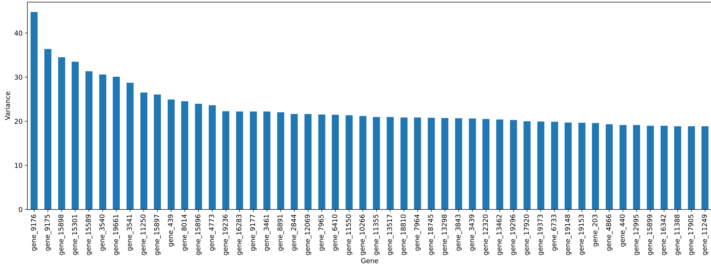
Top 50 Most Variable Genes
