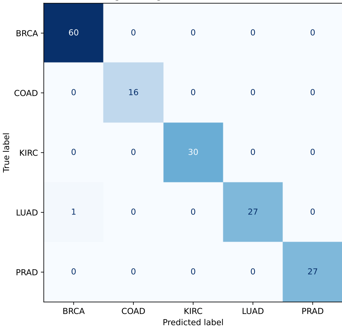
Logistic Regression Confusion Matrix
