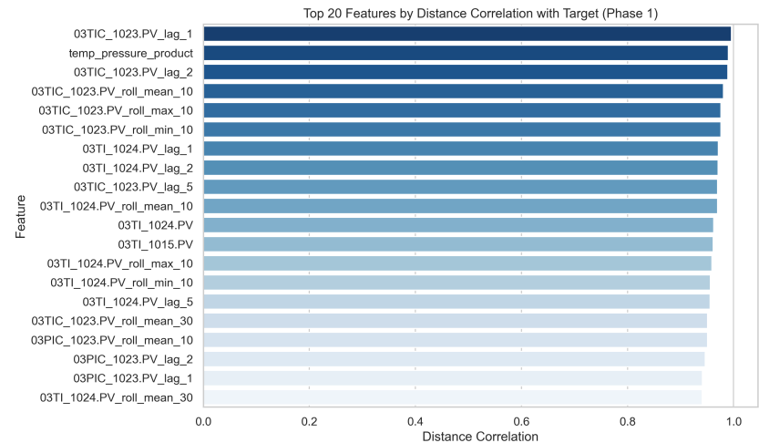
Figure 5: Top 20 Candidate Features by Distance Correlation with Target.
