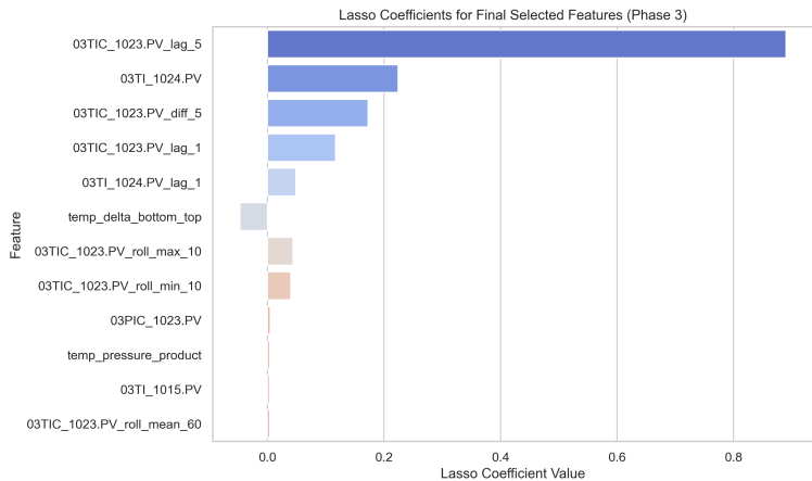
Figure 8: Phase 3 - Lasso L1 weights shrinking redundant and collinear features to zero.
