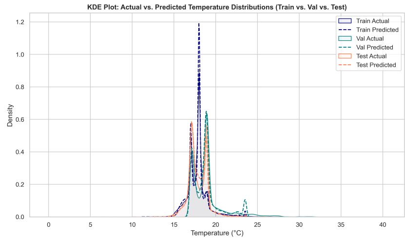
Figure 12: KDE Plot - Actual vs. Predicted Temperature Distributions (Train/Val/Test overlaid).
