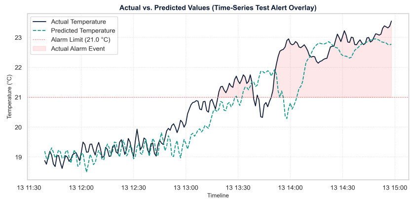
Figure 13: Time Series Plot - Actual vs. Predicted values on Y-axis against time (15 Min warning LSTM overlay).
