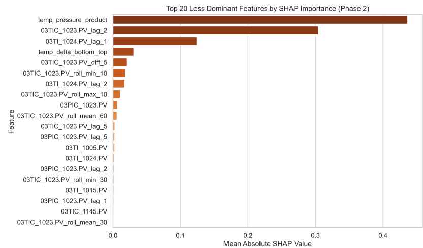
Figure 7: Phase 2 - SHAP Importance rankings for less dominant features.
