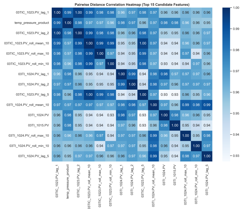
Figure 6: Pairwise Distance Correlation Heatmap (Top 15 Candidate Features).
