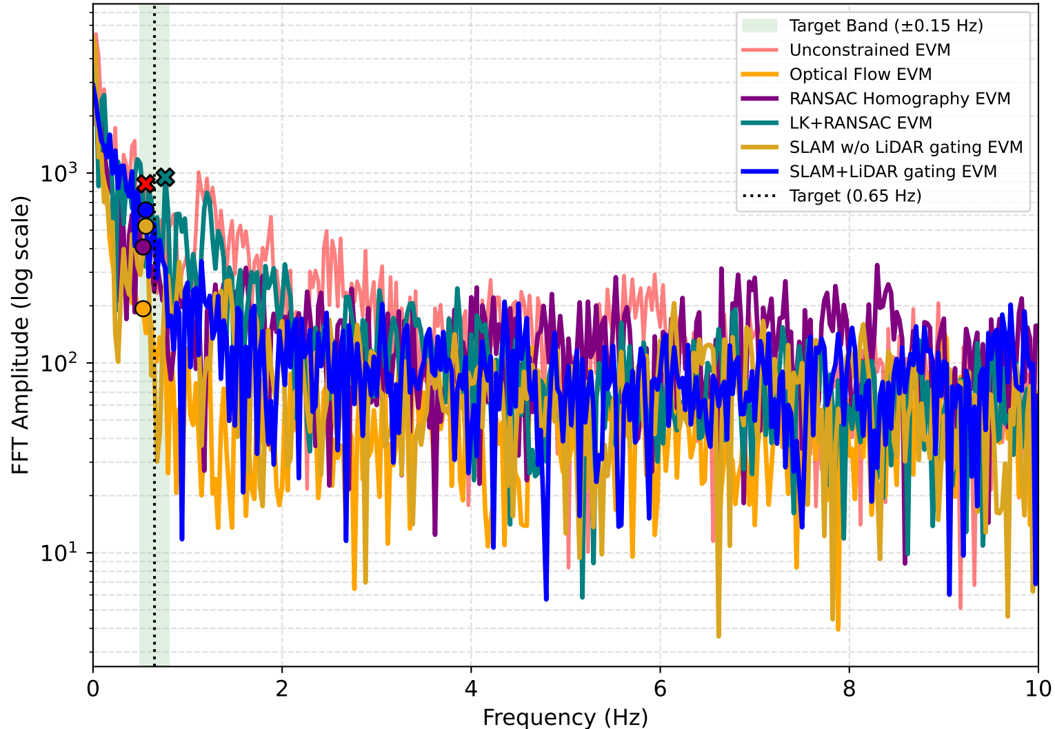
Vibration Spectrum Extraction Comparison (Log Scale, Target-Frequency Peaks Annotated)
