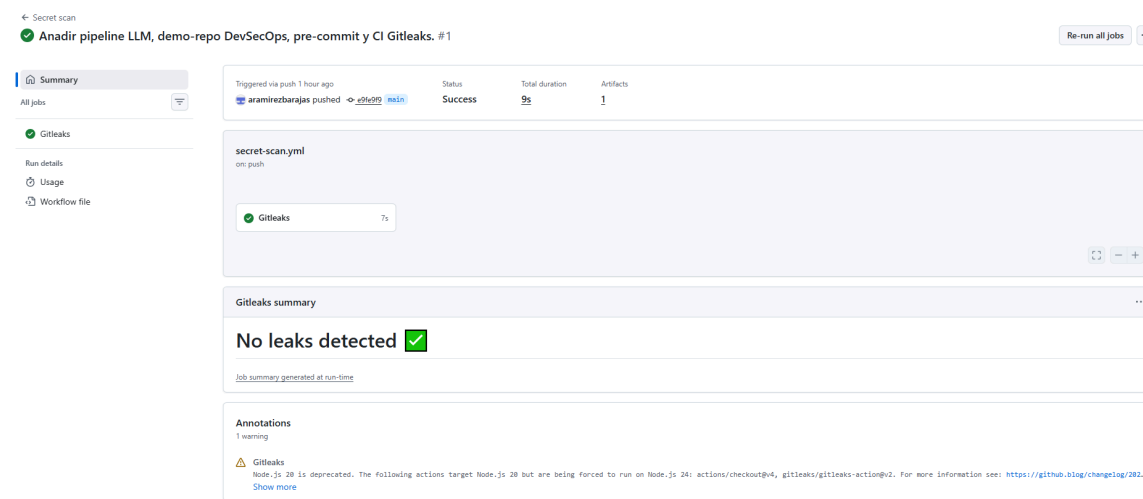
Figura B.2. Workflow secret-scan.yml en GitHub Actions: job Gitleaks en verde, No leaks detected.
