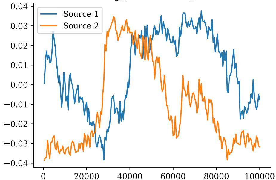
mixing_matrix MOCA_total
