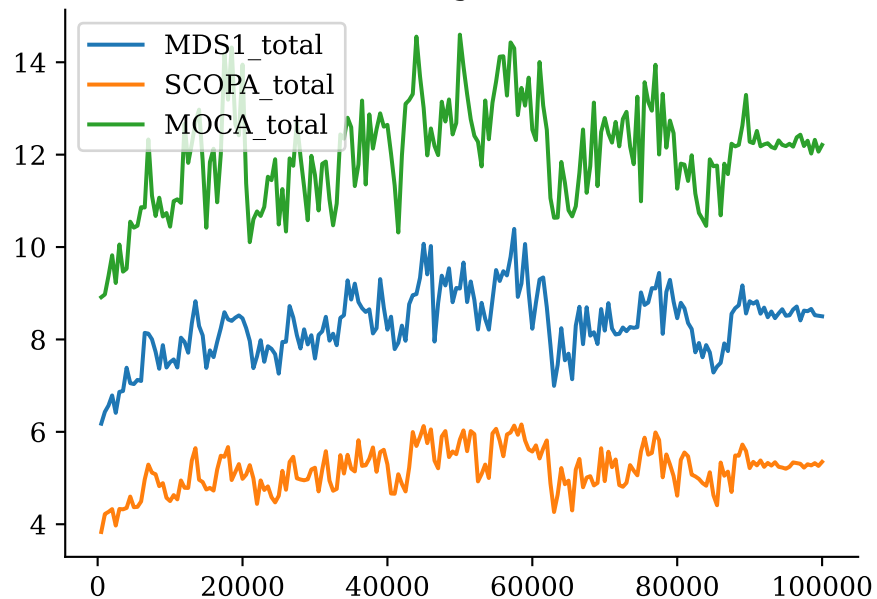
mixing_matrix SCOPA_total
