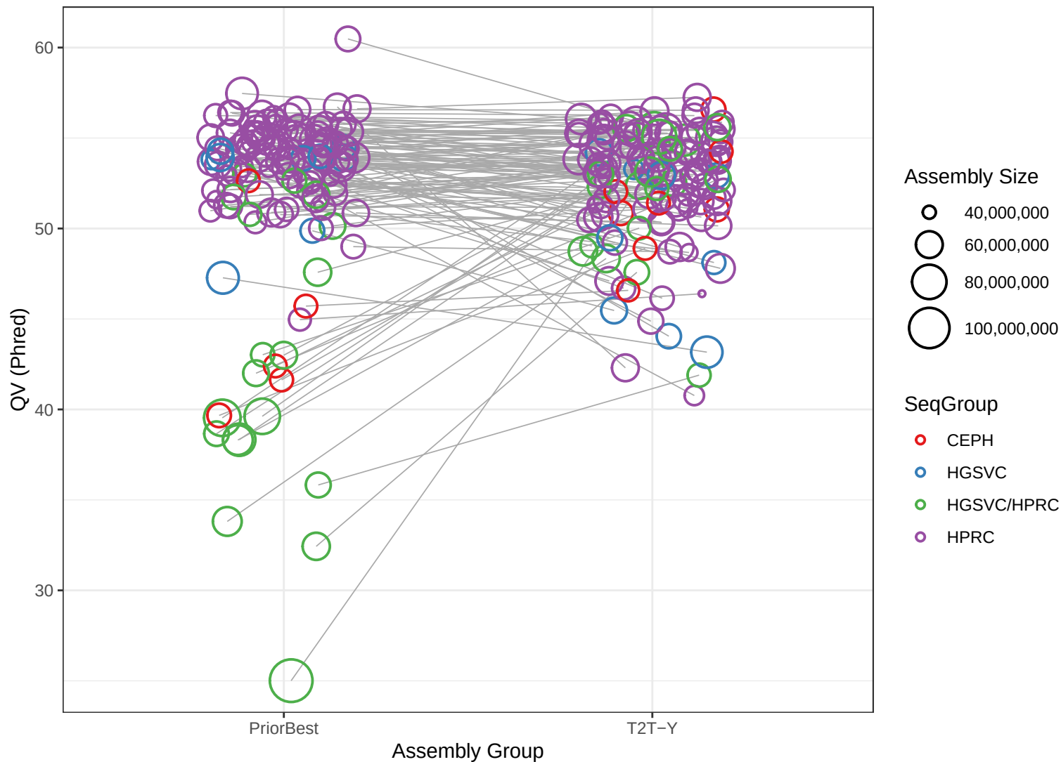
QV comparison across Y assemblies
