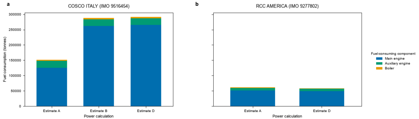
Figure 5. Fuel consumption by engine component and power estimate, 2017 to 2024, at a three-hour smoothing window.
