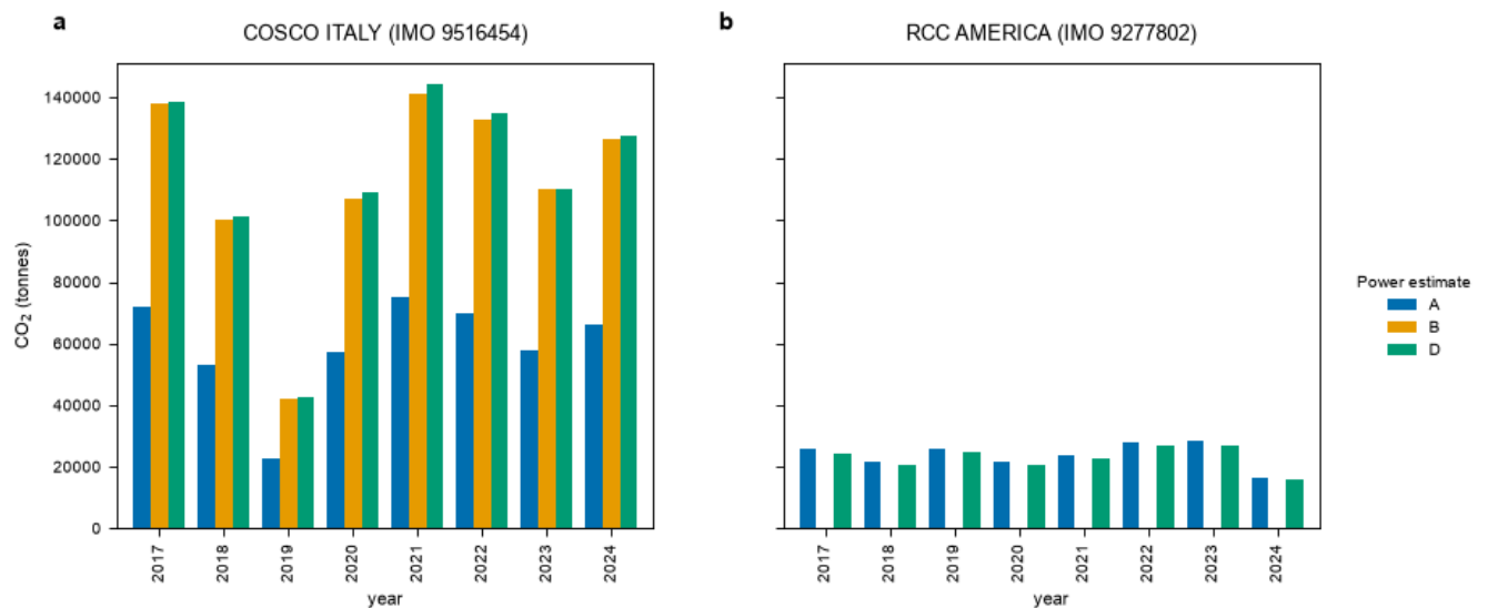
Figure 6. Annual CO 2 by power estimate, at a three-hour smoothing window.
