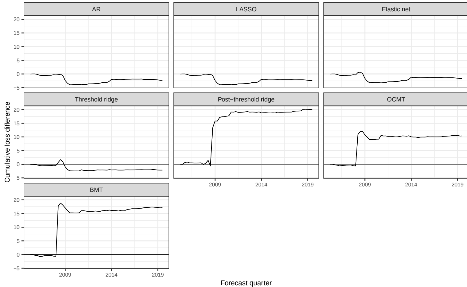
Cumulative Squared Loss Difference Relative to Ridge
