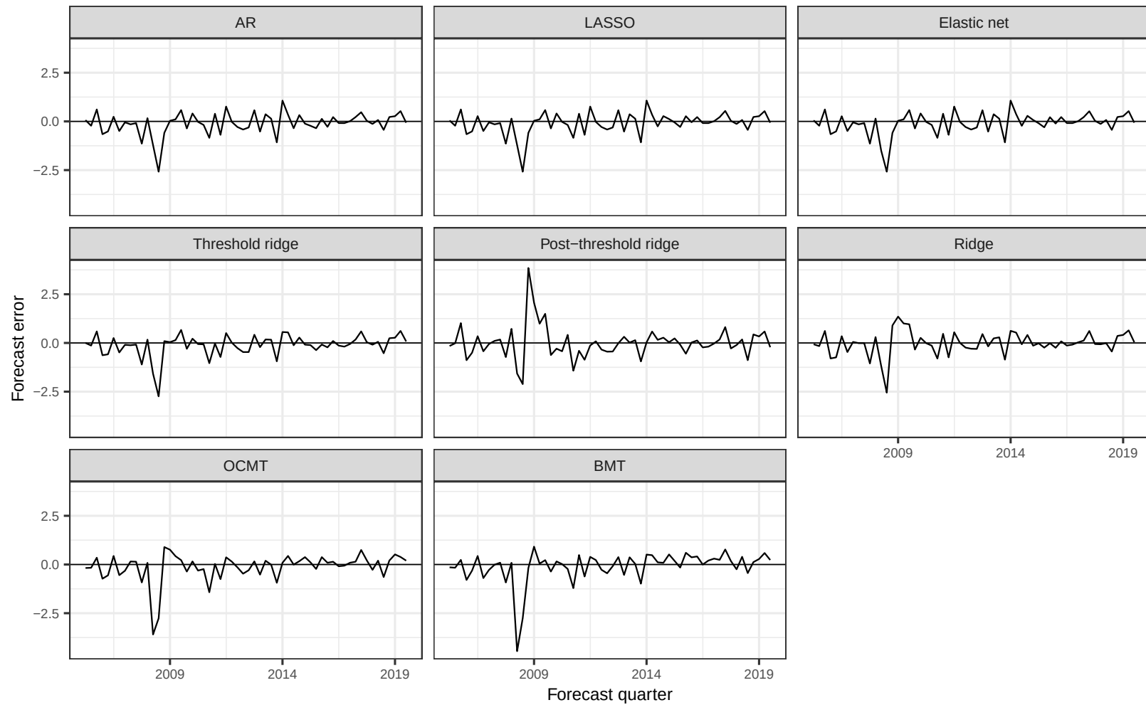
Forecast Errors over Time
