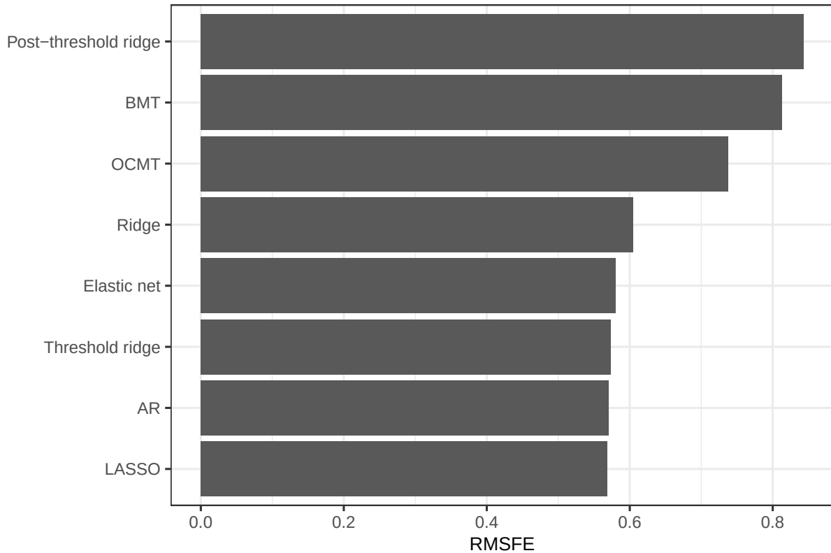
Root Mean Squared Forecast Error by Method
