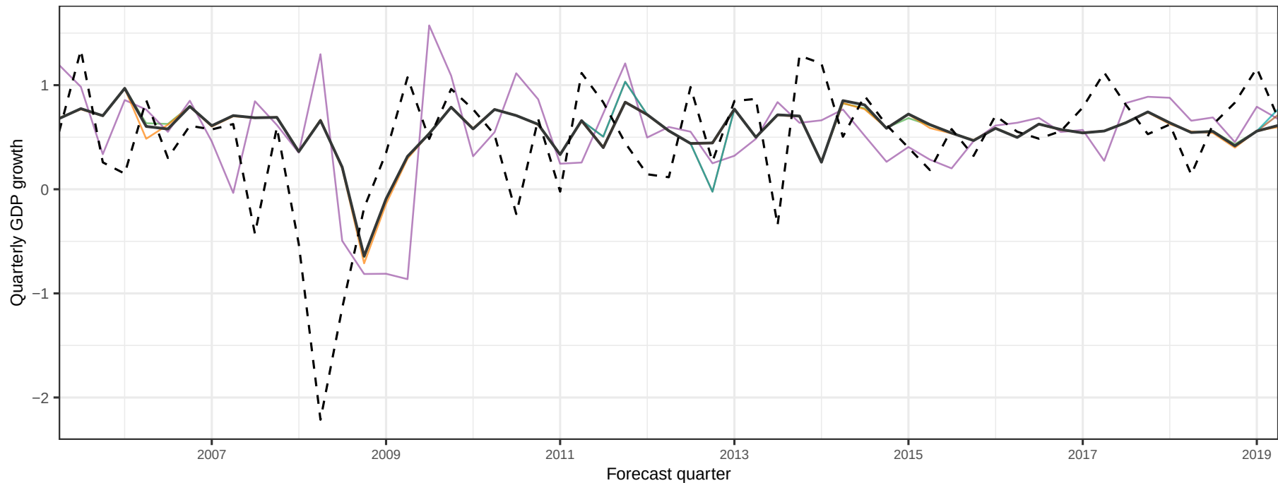
Forecasts and Squared Forecast Errors (h = 2)
