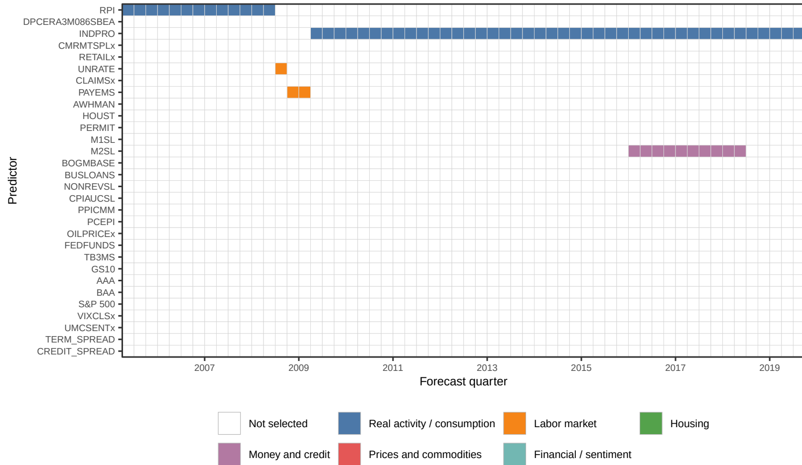
Variable Selection over Time for BMT
