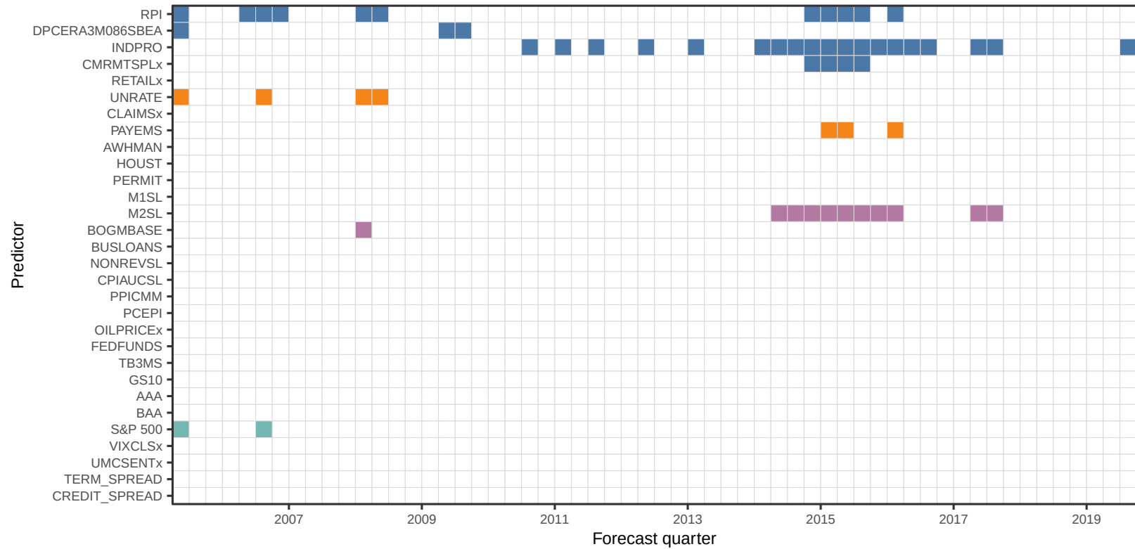
Variable Selection over Time for Elastic Net
