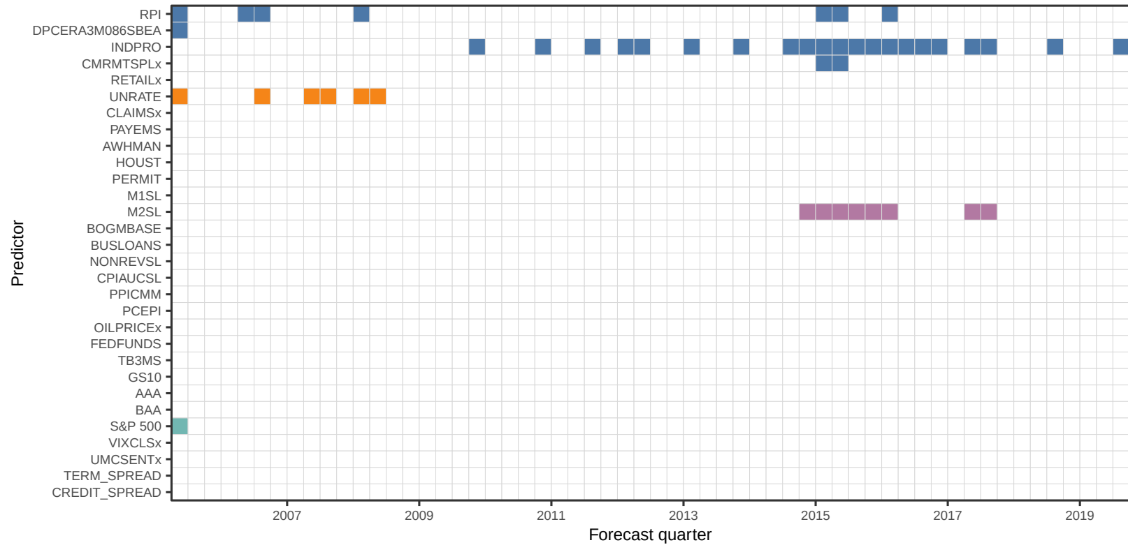
Variable Selection over Time for LASSO
