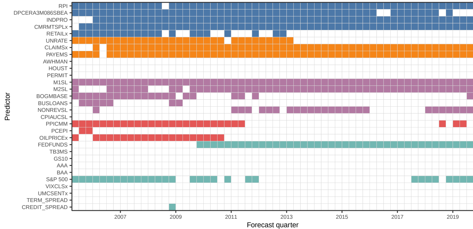
Variable Selection over Time for Post-Threshold Ridge
