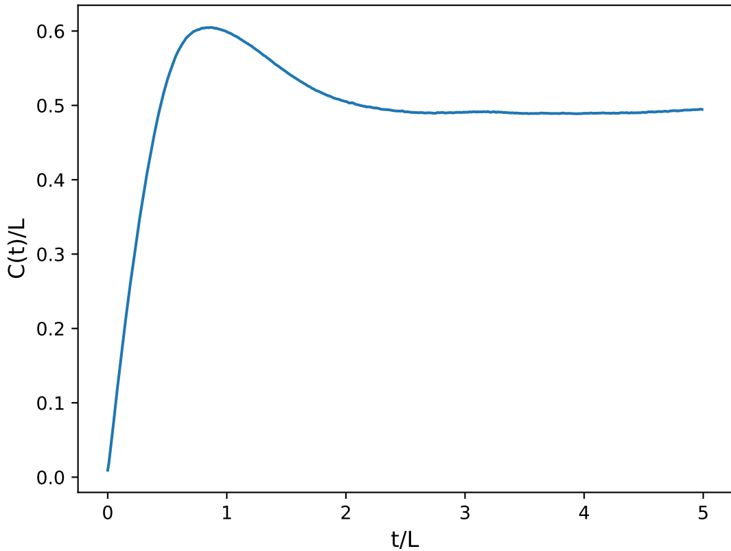
String Scattering, N=400
