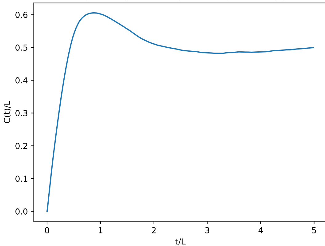
N=800, 4pt String Scattering involving HES (Regge limit)
