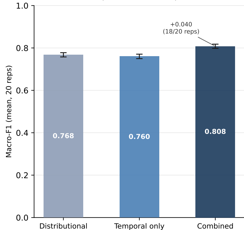
Binary classification (Control vs Patient)
