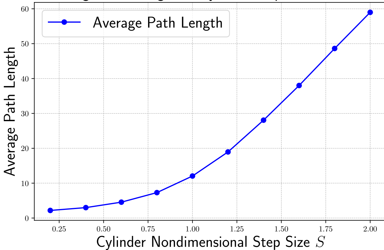
Average Path Length vs Cylinder Step Size for d = 2
