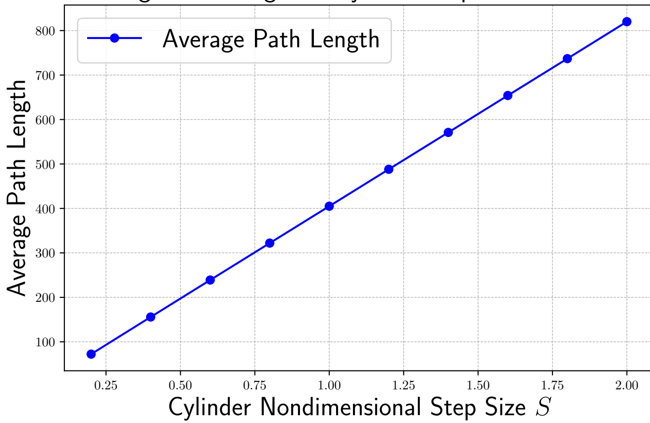
Average Path Length vs Cylinder Step Size for d = 20
