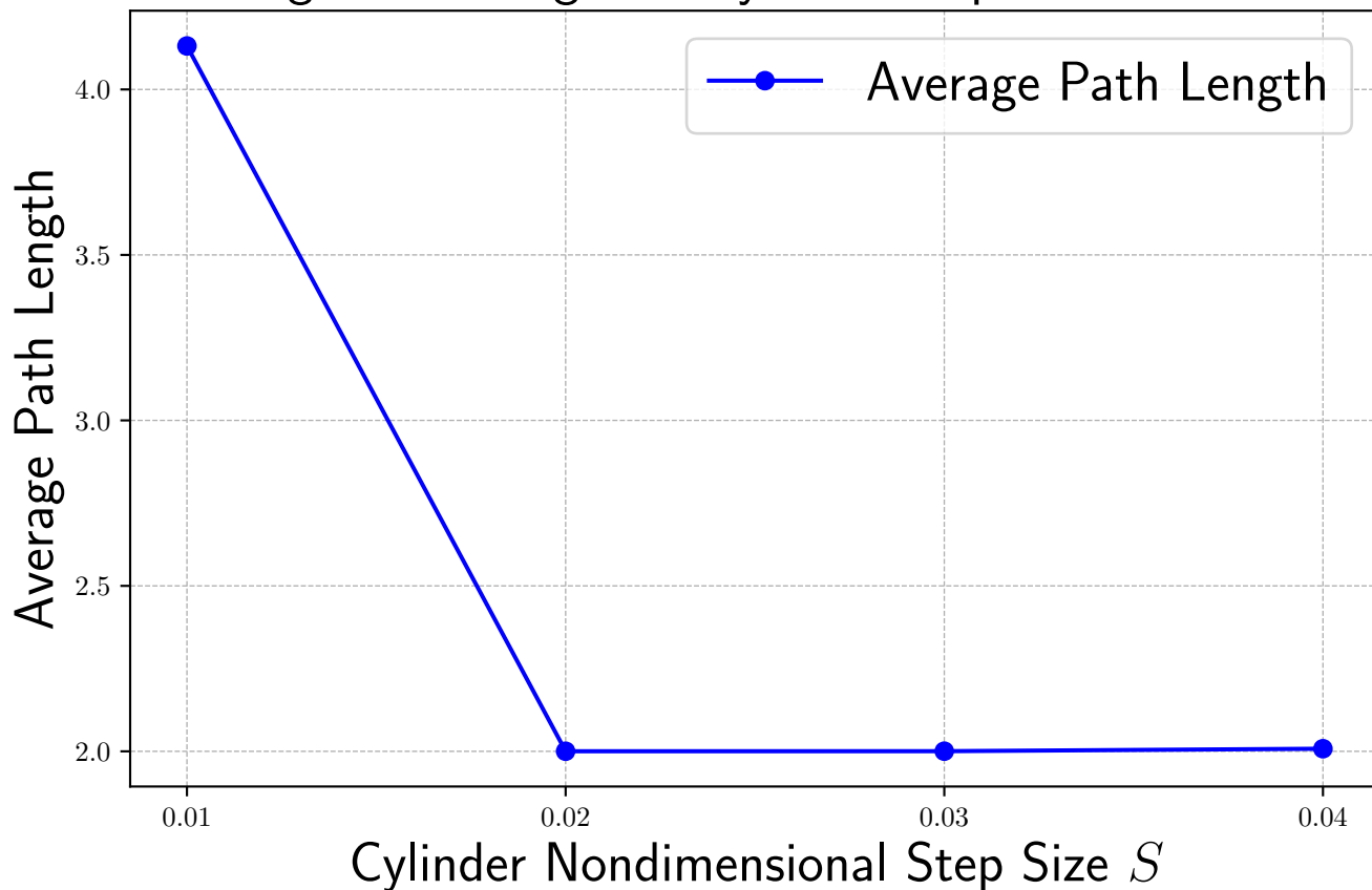
Average Path Length vs Cylinder Step Size for d = 10
