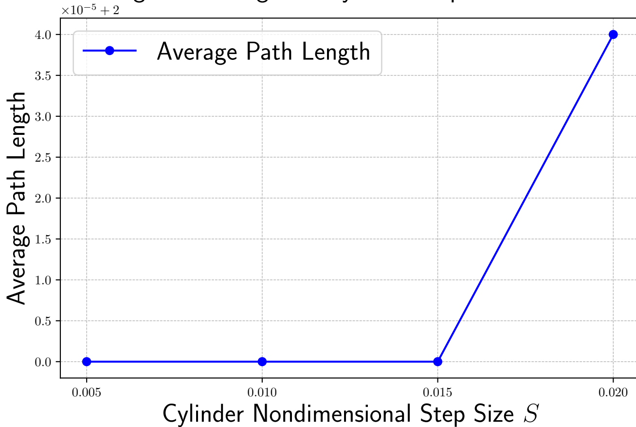
Average Path Length vs Cylinder Step Size for d = 15
