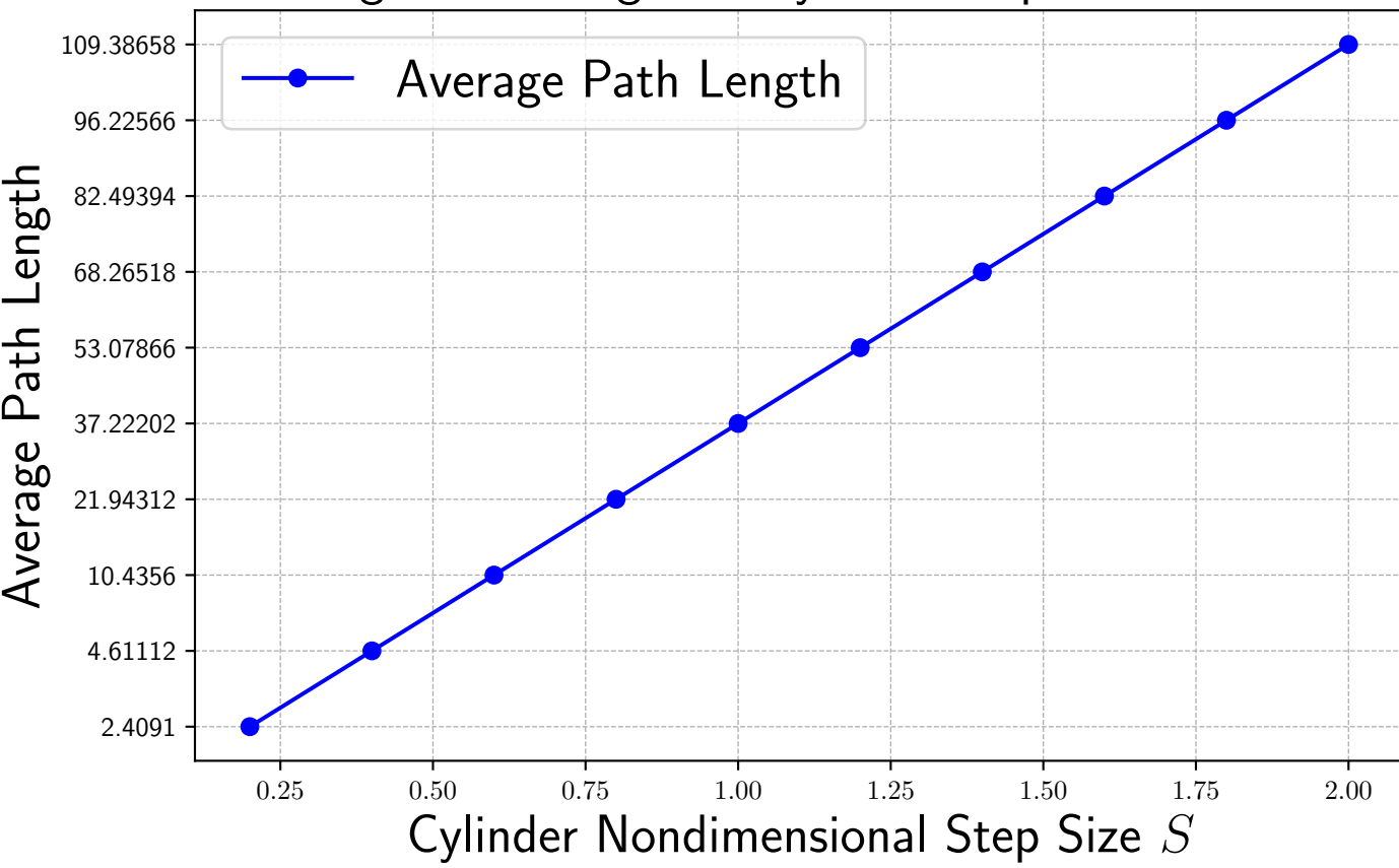
Average Path Length vs Cylinder Step Size for d = 3
