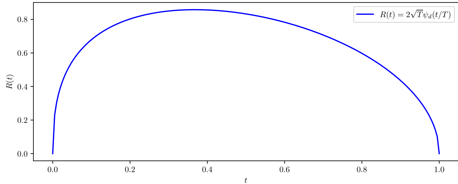
Radius Function R(t) for d = 2
