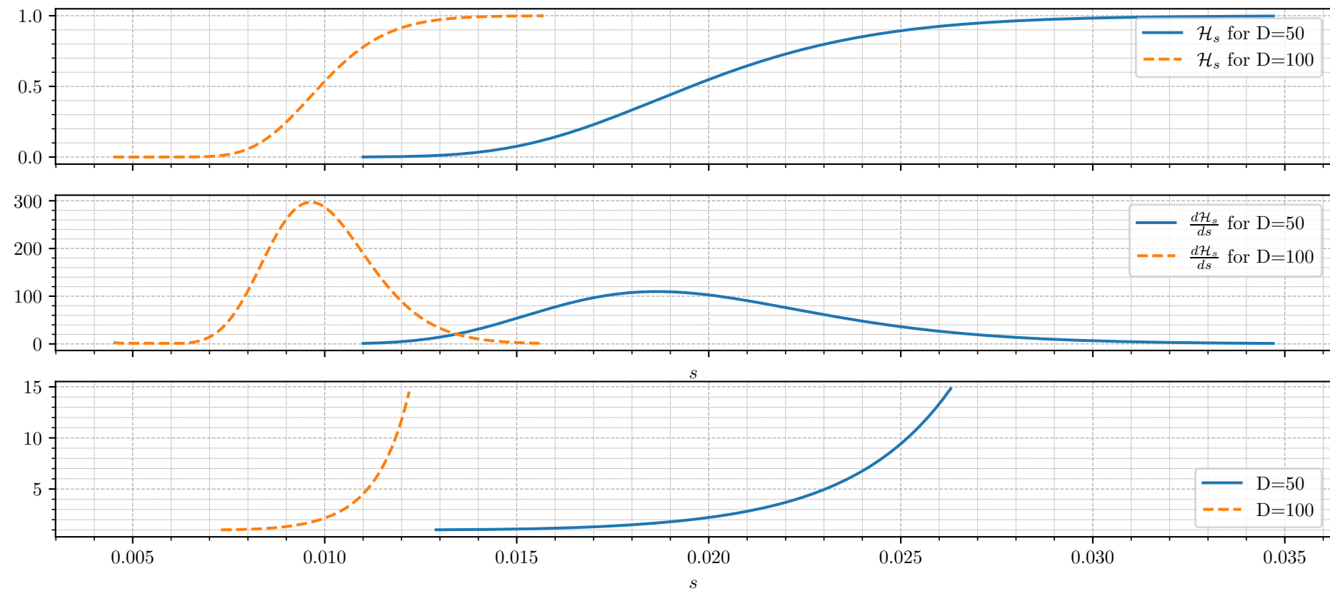
\mathcal{H}_s , its derivative, and number of steps for large dimensions
